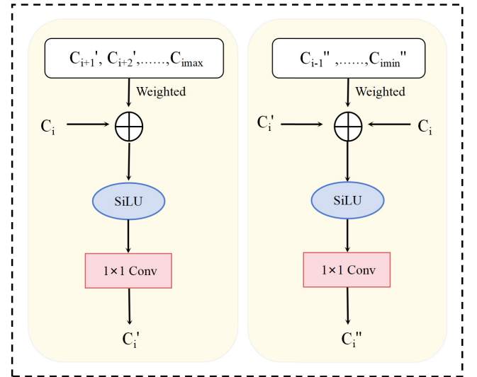
Fig. 2. Detailed fusion process of MDFFN feature map.
