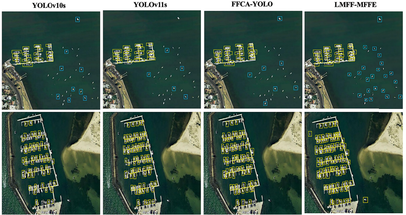
Fig. 8. Comparison of object detection visualization results for different detection methods.
