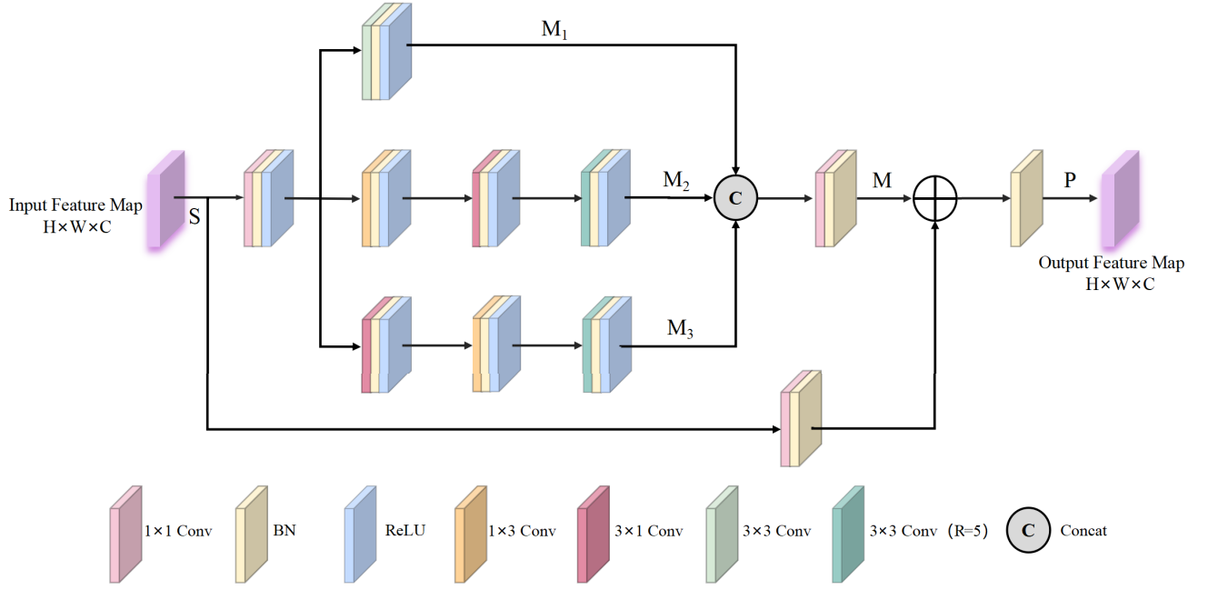
Fig. 3. Architecture of MRFFE.
