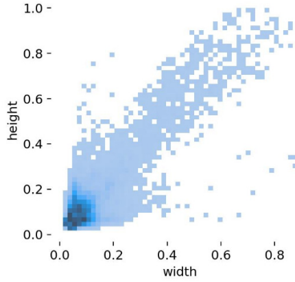
Fig. 6. SIMD dataset size distribution.
