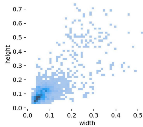
Fig. 5. NWPU VHR-10 dataset size distribution.
