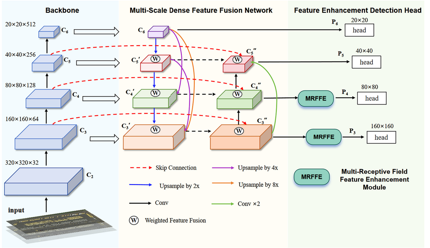
Fig. 1. Overall LMFF-MFFE architecture.
