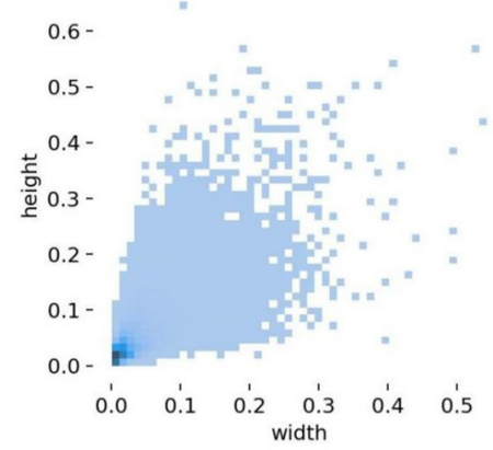
Fig. 4. VisDrone2019 dataset size distribution.
